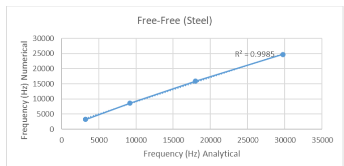
Fig. 5. First 4 modes for Free-Free steel beam analytical Vs numerical.
